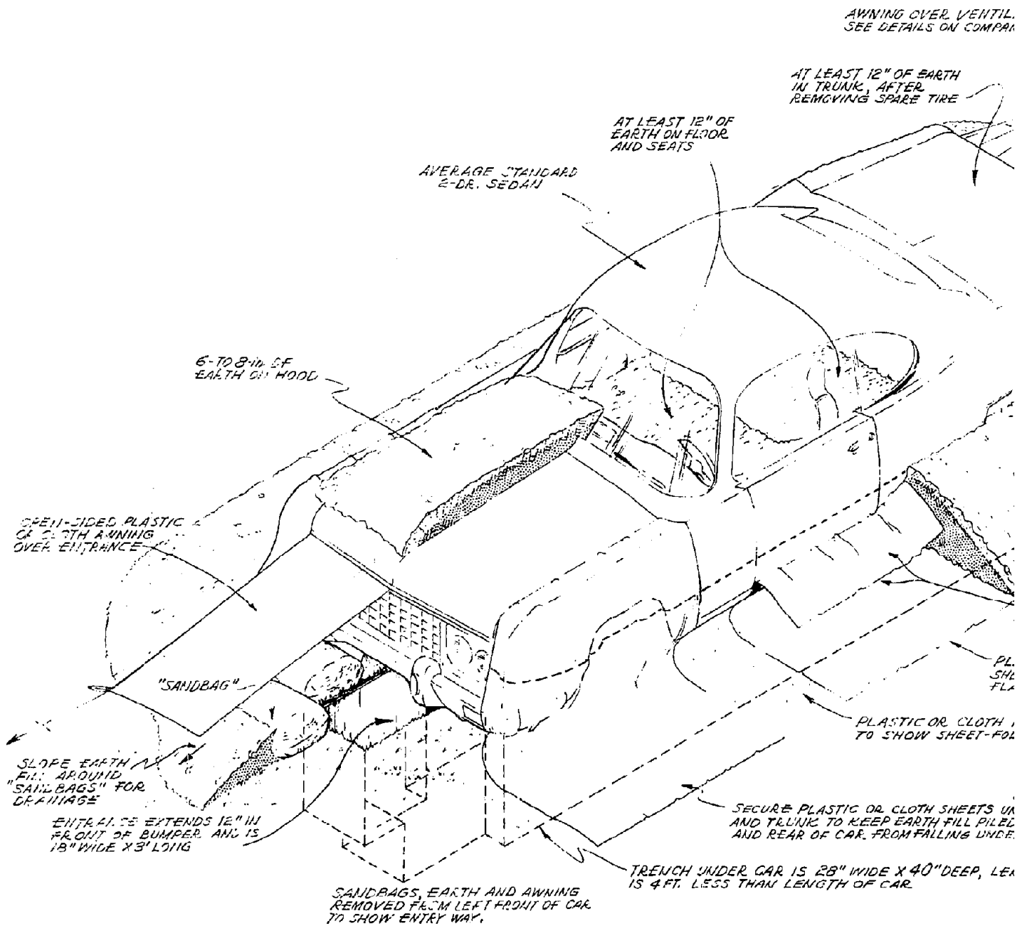
Fig. A-13.1. Car-Over-Trench Shelter, Pictorial View.
